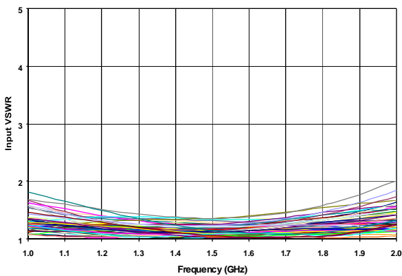
Figure 5. Input VSWR Over All Phase States
